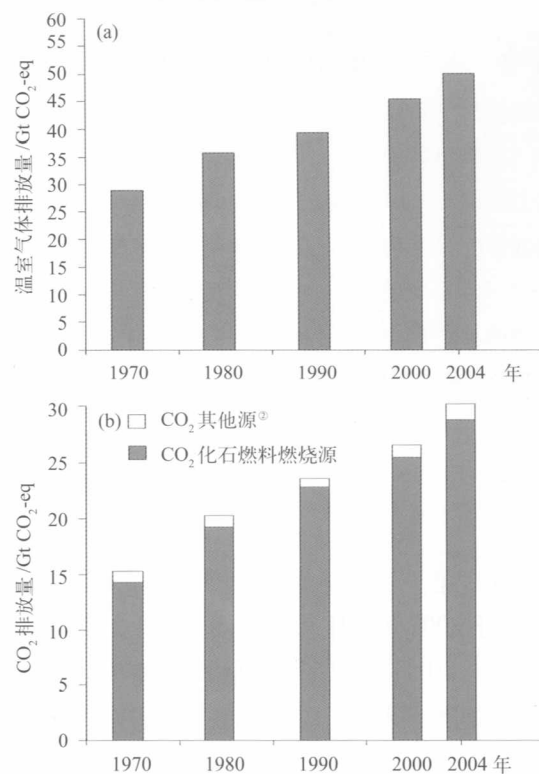
图1 以全球增温潜力计算的温室气体(a)及 \text{CO}_2 (b)排放量变化 Fig. 1 Global warming potential weighted global greenhouse gas (a) and \text{CO}_2 (b) emissions in 1970-2004
